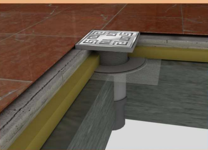
Hisar Series / Bottom Outlet
