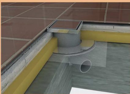
Abant Series / Side Outlet
