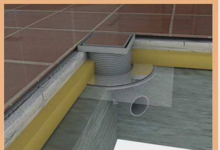
Topkapı Series / Side Outlet
