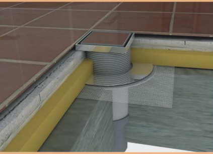
Abant Series / Bottom Outlet
