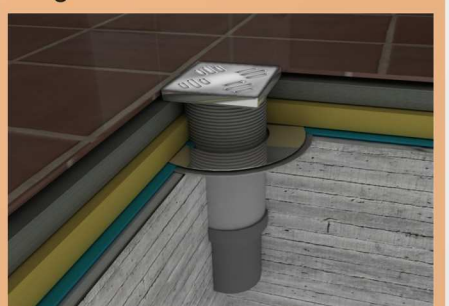
İlgaz Series / Bottom Outlet
