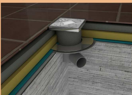
İlgaz Series / Side Outlet
